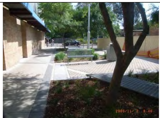
a) Pervious pavers and rain garden, Guildford Lane, Guildford.
